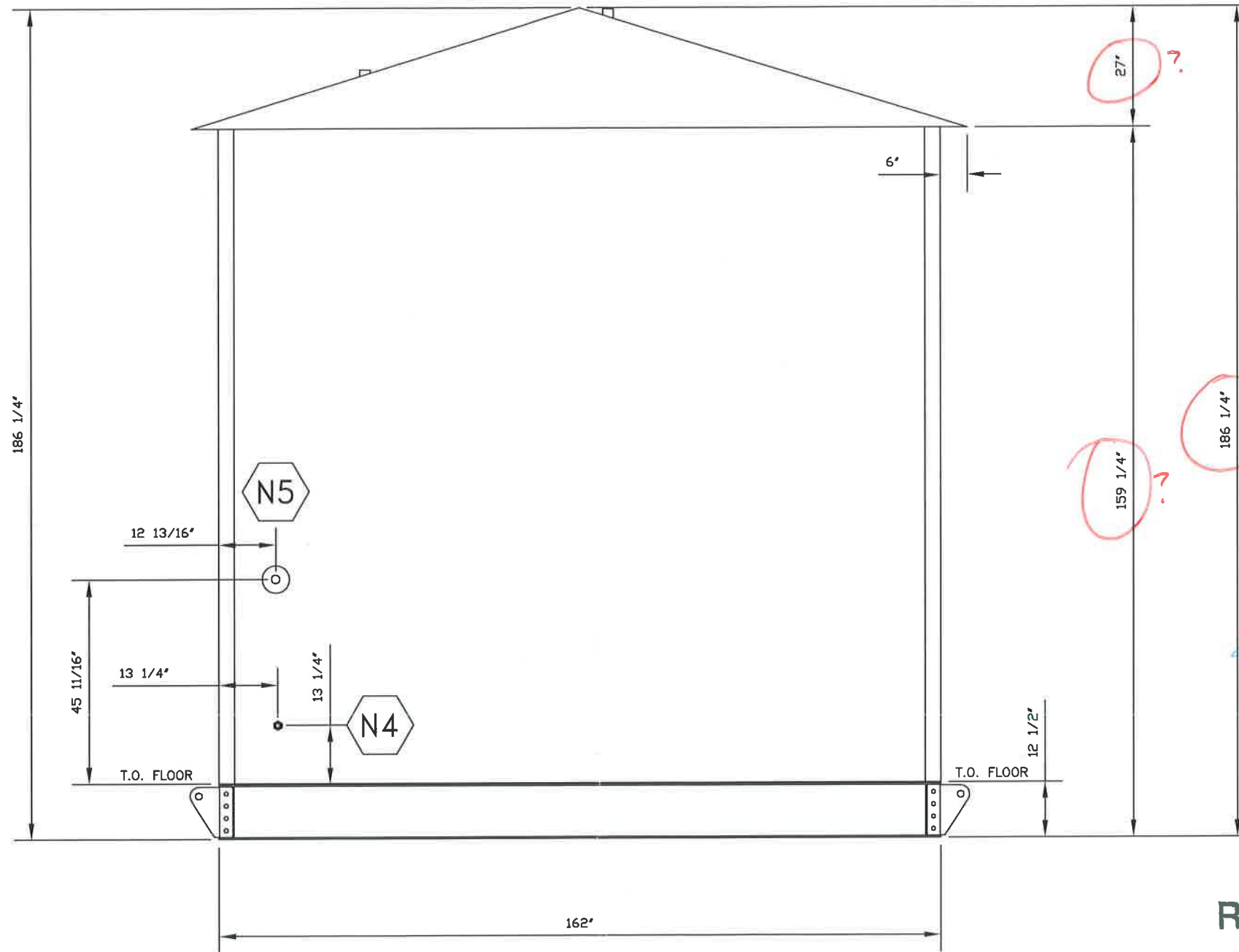
SECTION C SCALE 1:30
