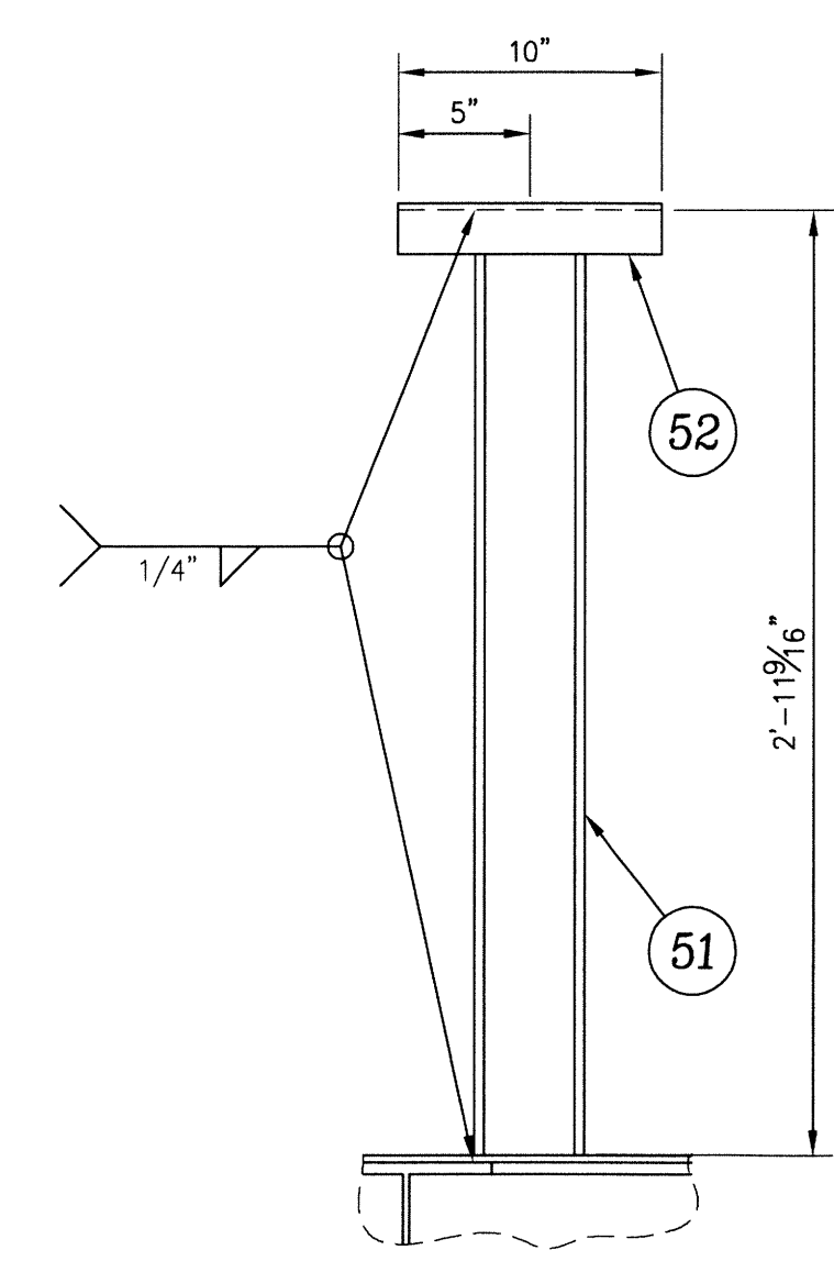
PS 1 DETAIL SCALE 1 1/2"=1'-0" (1 REQ'D)
